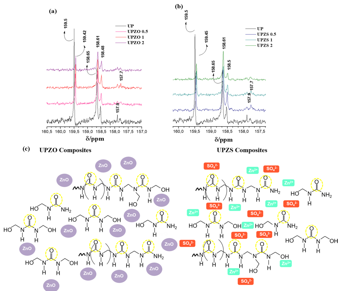
Figure 6. Amplification spectra of ^{13}\text{C} NMR 160–157 ppm of composites (a) UPZO and (b) UPZS solubilized in \text{DMSO}-d_6 and molecular structure proposed for the interaction of Zn particles with the polymers as well as the different medium of carbonyl groups. Molecular structure created using software Microsoft PowerPoint 2016 version.
