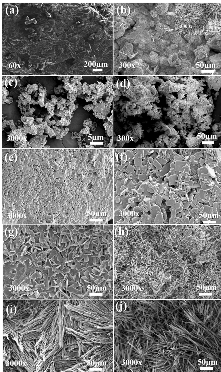
Figure 1. SEM images with its magnifications of (a) pure urea, (b) pure polymer UF, (c) ZnO, (d) ZnSO 4 , (e) UFZO 0.5, (f) UFZO 1, (g) UFZO 2, (h) UFZS 0.5, (i) UFZS 1 and (j) UFZS 2. (UF=pure polymer, UFZO = composites with ZnO and UFZS composites with ZnSO 4 ).
