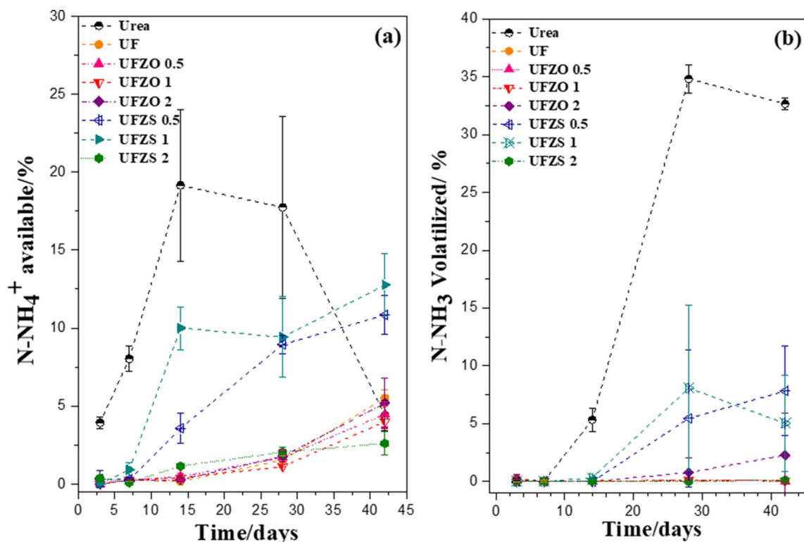
Figure 8. N recovery from the fertilizers as (a) \text{N-NH}_4^+ available and (b) \text{N-NH}_3 volatilized for each fertilizer treatment over the 42-day incubation period.
